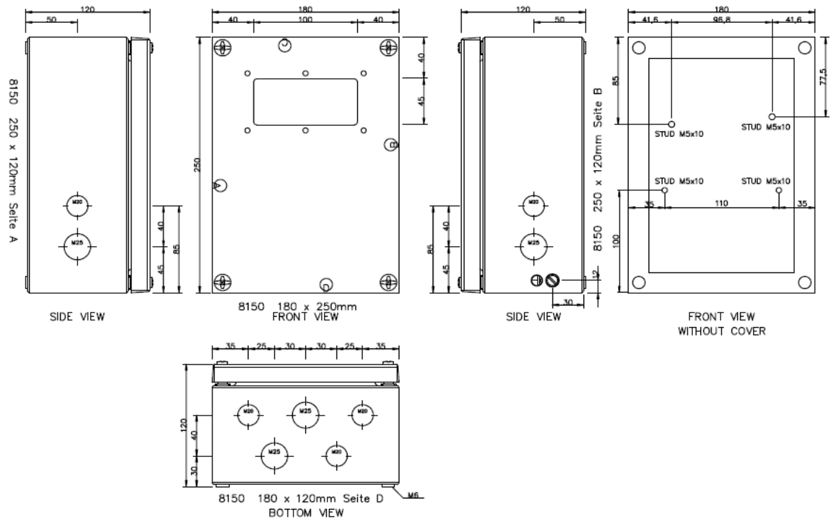
Figure 4: TraceNet ECM Dimensions
